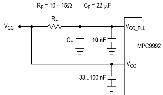
Figure 4. V_{CC\_PLL} Power Supply Filter
